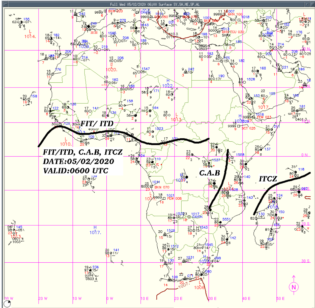
Tabulated positions of the ITD: 05 th FEBRUARY 2020
